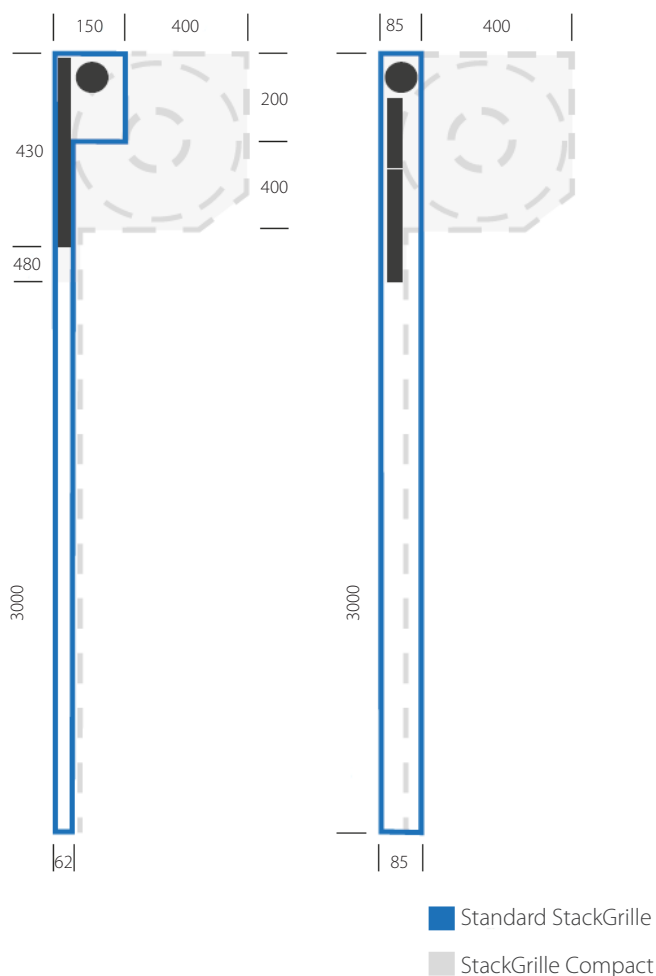
Standard StackGrille StackGrille Compact
